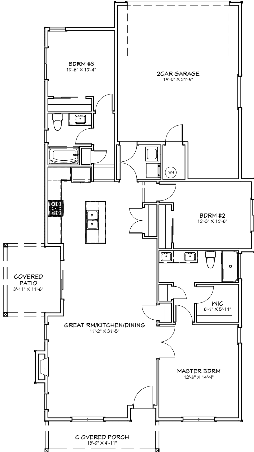
FLOOR PLAN 1517 SQ FT
