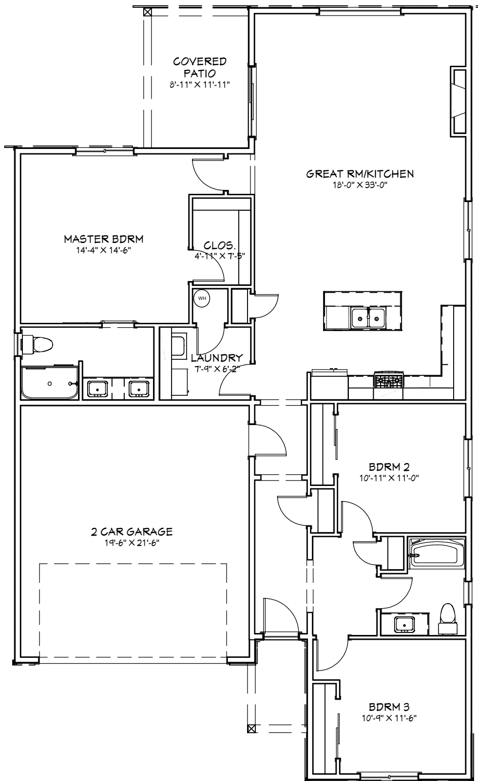
FLOOR PLAN 1634 SQ FT
